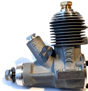
Fora 2.5cc (.15cid) F2E-Diesel $239.95
